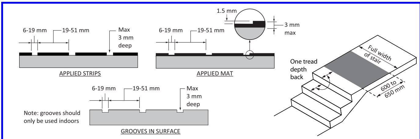
Figure A-3.8.3.9.(5) Tactile walking surface indicators
