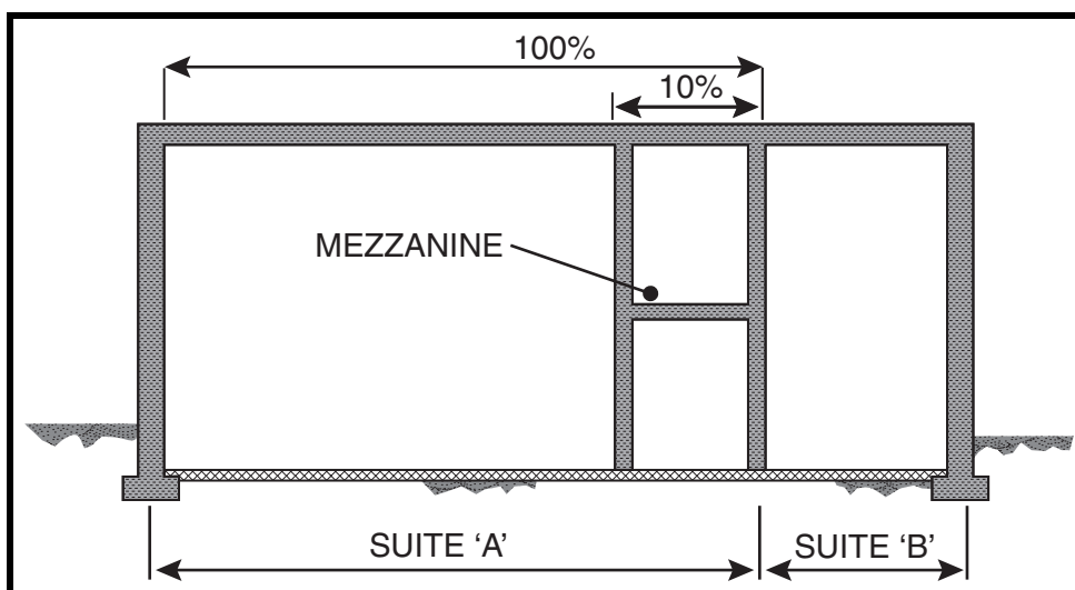
Figure A-3.2.1.1.(4)-C Mezzanines in Multi-Tenant Suites
