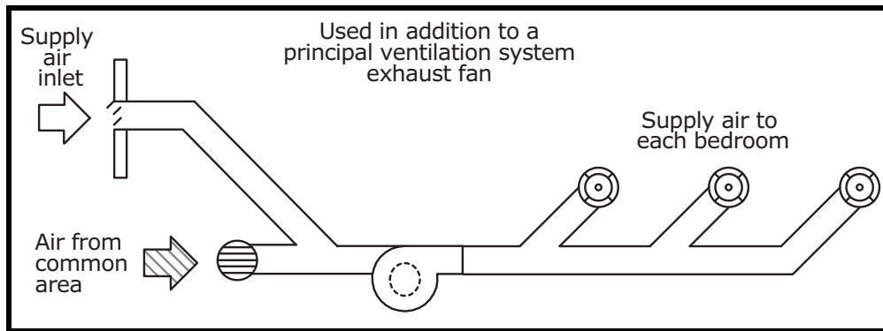
Figure A-9.32.3.4.(5)(b)(ii) Central Recirculation System Supply Air Distribution
