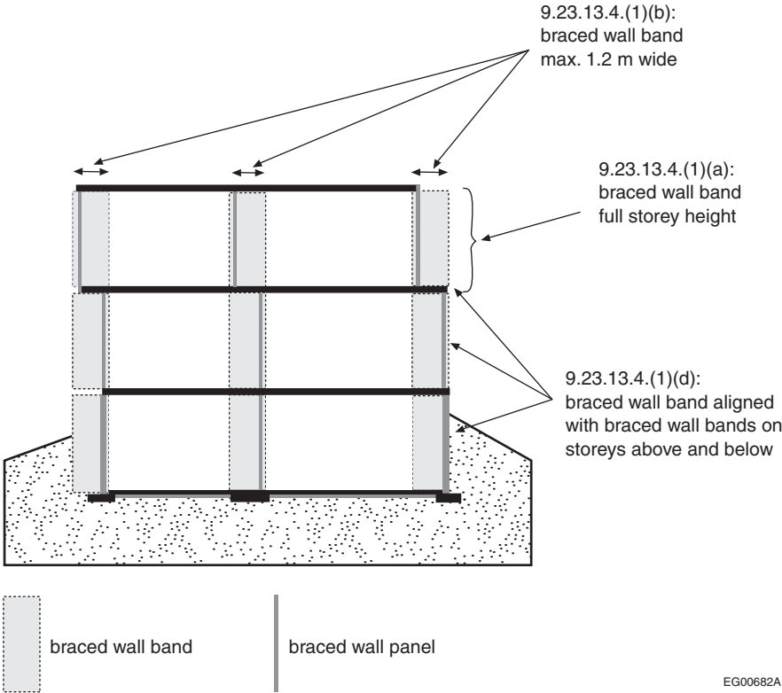
Figure A-9.23.13.4.-A Braced wall bands in an example building section [Clauses 9.23.13.4.(1)(a), (b) and (d)]
