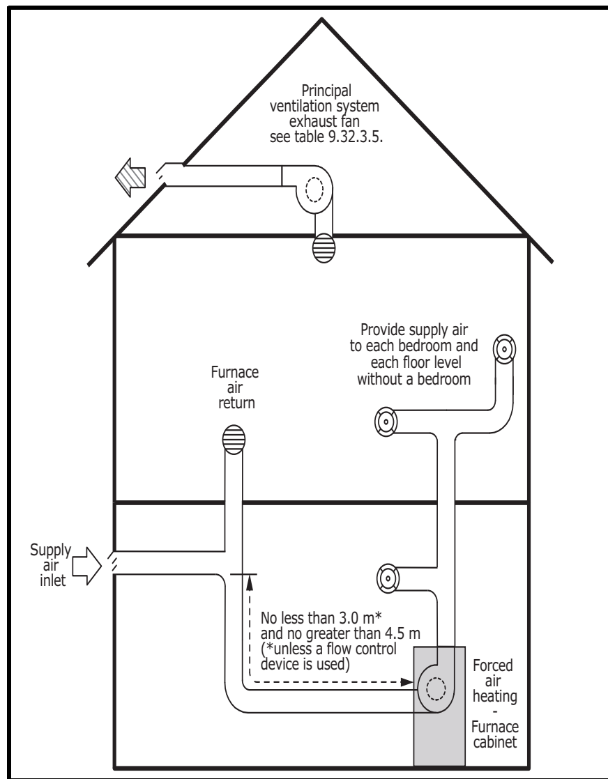
Figure A-9.32.3.4.(2) Forced-Air Heating System Supply Air Distribution
