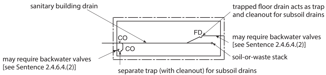
(a) Connections to sanitary drainage system (plan view)
