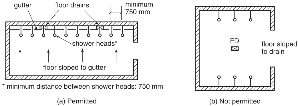
Figure A-2.2.3.(3) Shower Drainage (Plan View)
