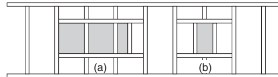
Figure A-9.23.10.6.(3)-A Single studs at openings in non-loadbearing interior walls
