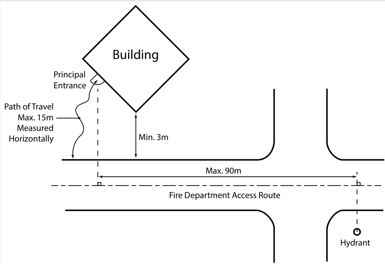
Figure A-3.2.5.5.-D
