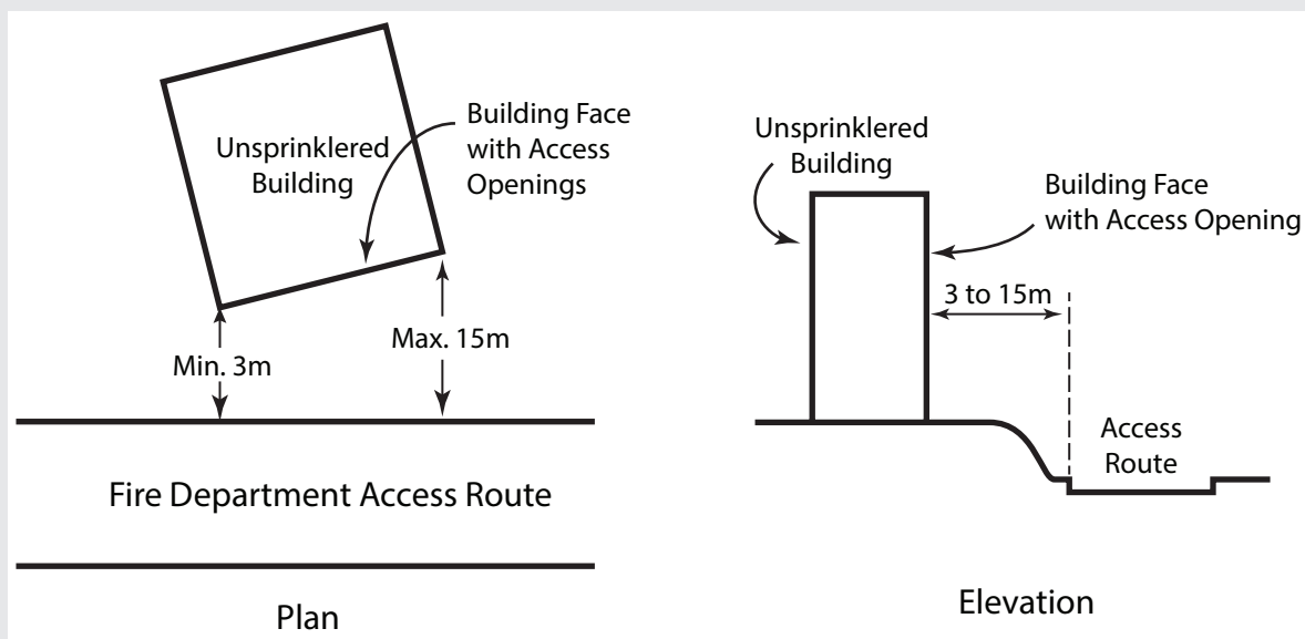
Figure A-3.2.5.5.-B
