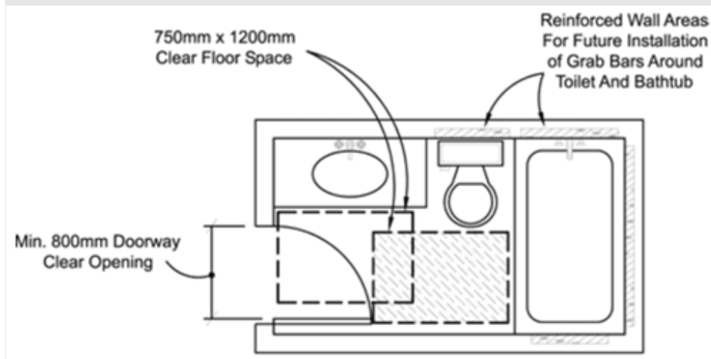
Figure A-3.8.3.1.(2)(i)-B Enhanced Accessibility Direct Approach
