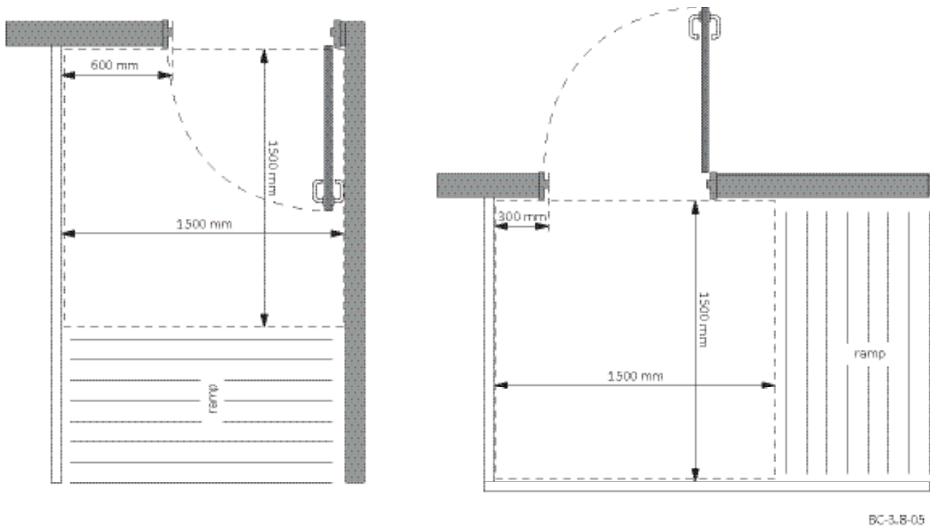
Figure A-3.8.3.5.(1)(c) Landing design at doorways leading to ramps
