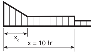
Distribution of snow load, S
