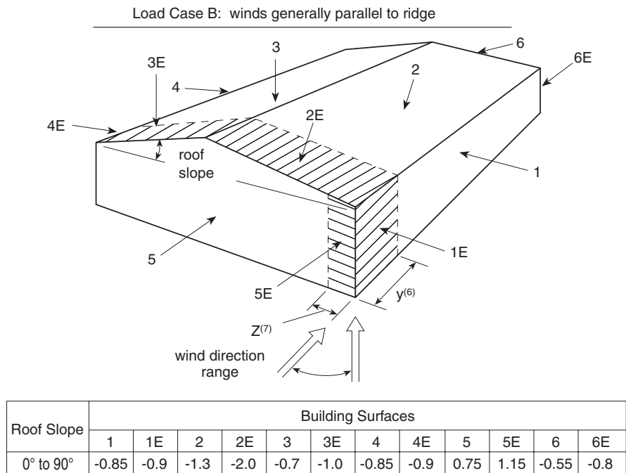
Figure 4.1.7.6.-A External peak values of C_p C_g for primary structural actions arising from wind load acting simultaneously on all surfaces of low buildings ( H \leq 20 m) Forming Part of Sentence 4.1.7.6.(2)
