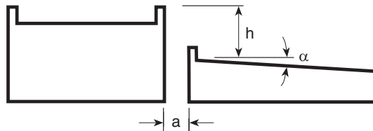
Distribution of snow load, S
