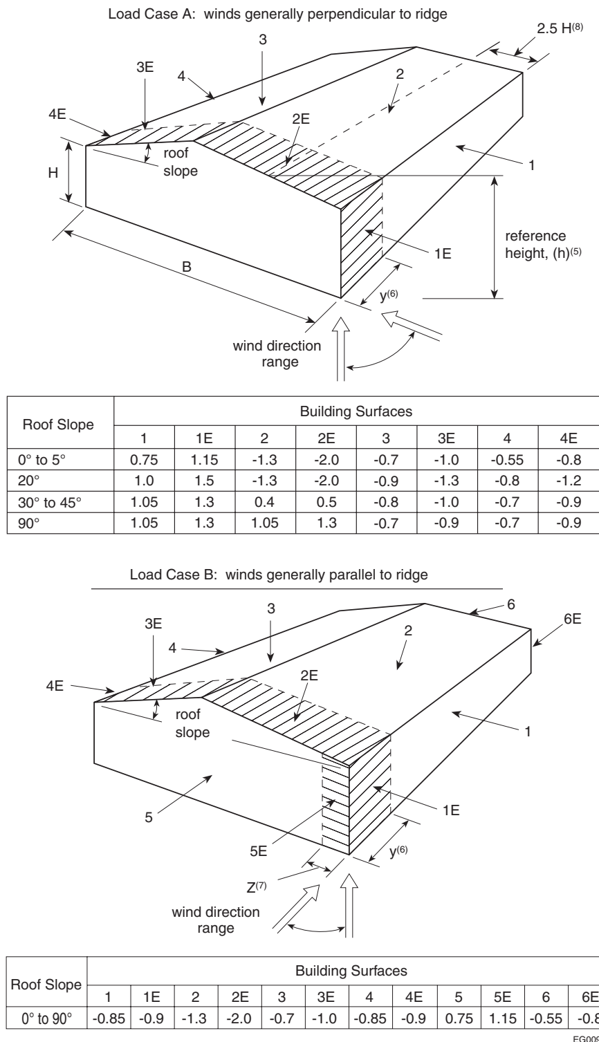
Figure 4.1.7.6.-A External peak values of C_p C_g for primary structural actions arising from wind load acting simultaneously on all surfaces of low buildings ( H \leq 20 m)
