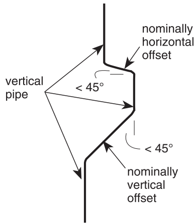
(a) Elevation view of vertical pipe
