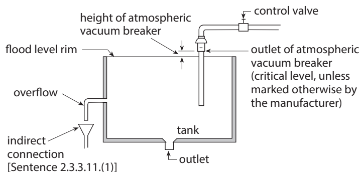
Figure A-2.6.2.10.(2) Installation of Atmospheric Vacuum Breakers
