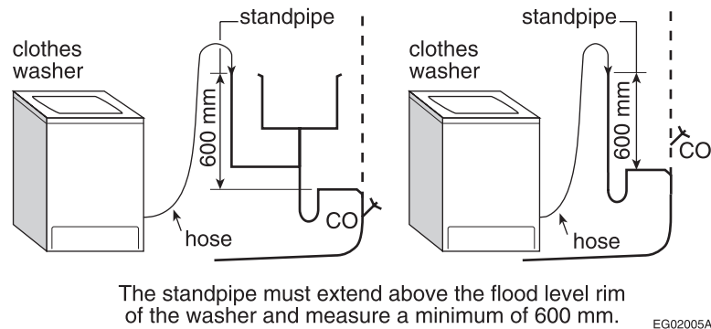
Figure A-2.4.9.3.(3) Standpipe Installation for Clothes Washers
