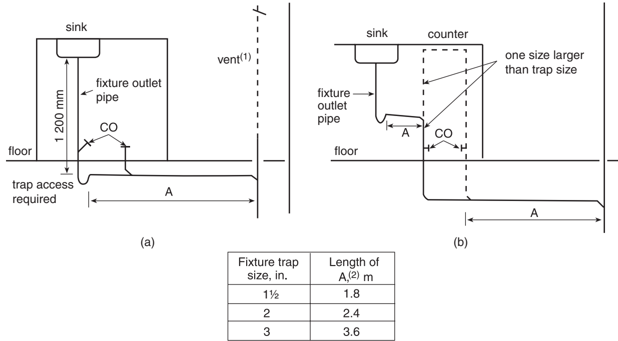
Figure A-2.4.8.2.(1) Island Fixture Installation (3)
