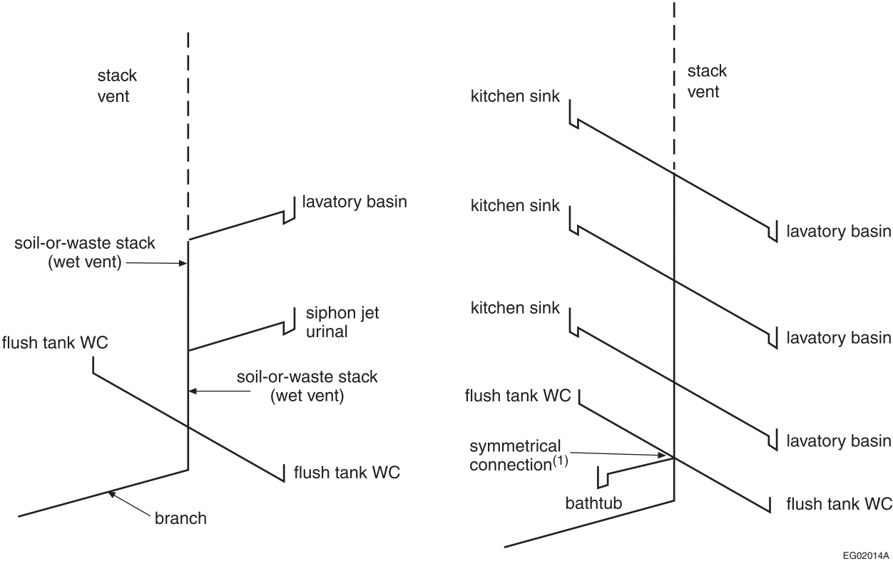
Figure A-2.5.2.1.-B Example of Wet Venting Described in Clause 2.5.2.1.(1)(c) Note to Figure A-2.5.2.1.-B:
