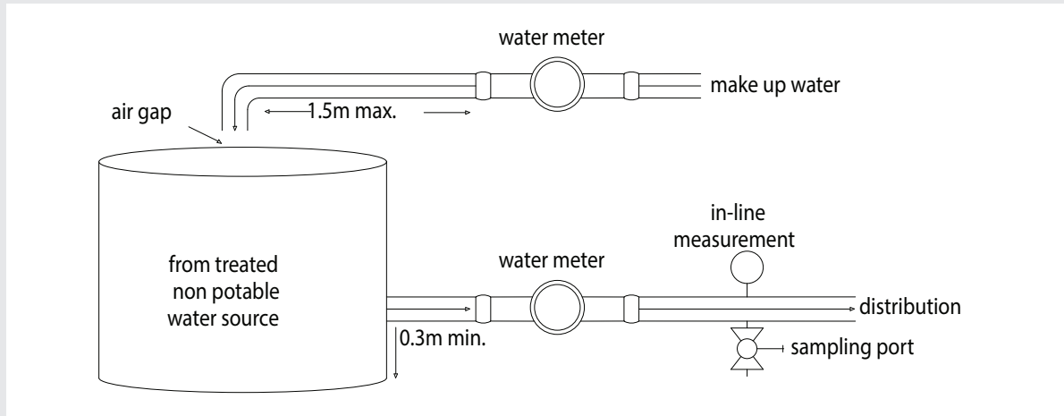
Figure A-2.7.6.4., 2.7.6.5. and 2.7.6.6. Schematic Example for a Non-potable Water System
