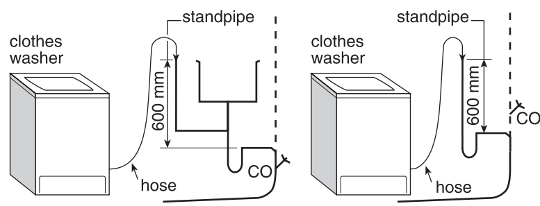
Figure A-2.4.9.3.(3) Standpipe Installation for Clothes Washers
